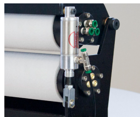
Adjustable roller pressure.
